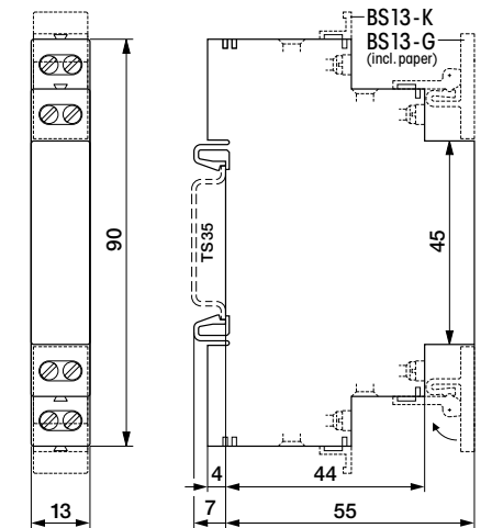
Dimension
