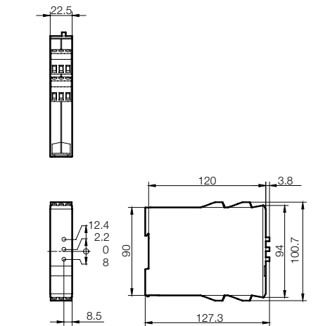
fig. 2. Dimensions (mm)
