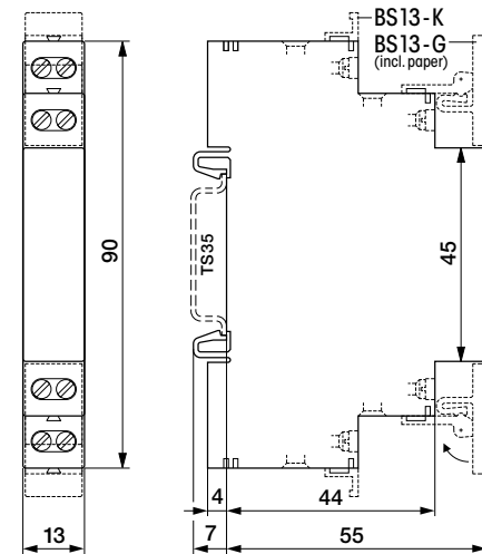
Dimensions (mm)
