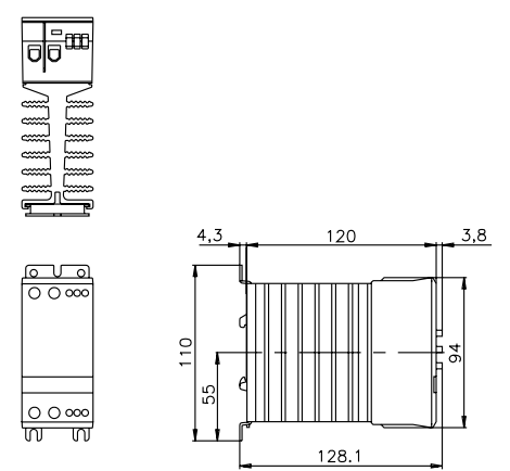
fig. 2. Dimensions (mm)
