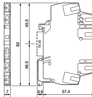
fig. 2. Dimensions (mm)
