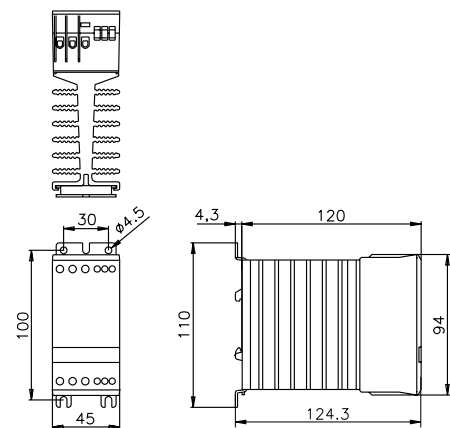
fig. 2. Dimensions (mm)
