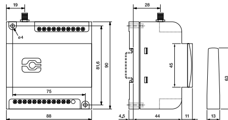
fig. 2. Dimensions (mm)
