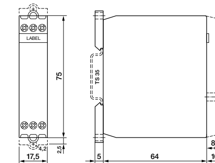
fig. 2. Dimensions (mm)
