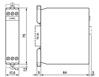
fig. 2. Dimensions (mm)
