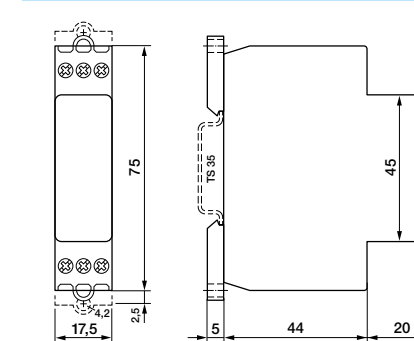
fig. 2. Dimensions (mm)
