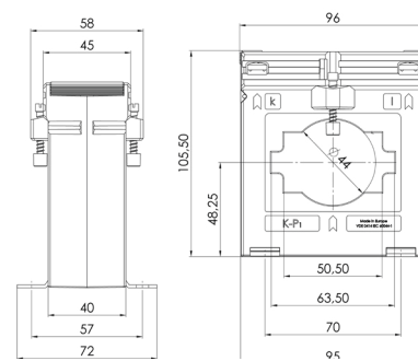
fig. 2. Dimensions (mm)
