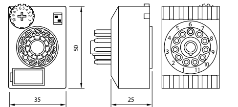
fig. 2. Dimensions (mm)
