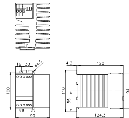
fig. 2. Dimensions (mm)
