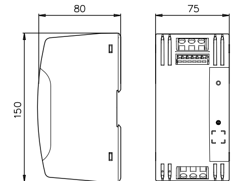
fig. 2. Dimensions (mm)
