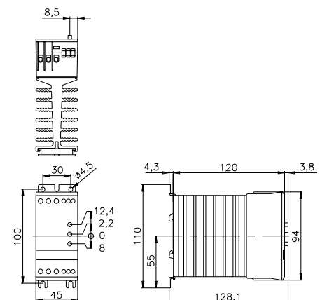
fig. 2. Dimensions (mm)
